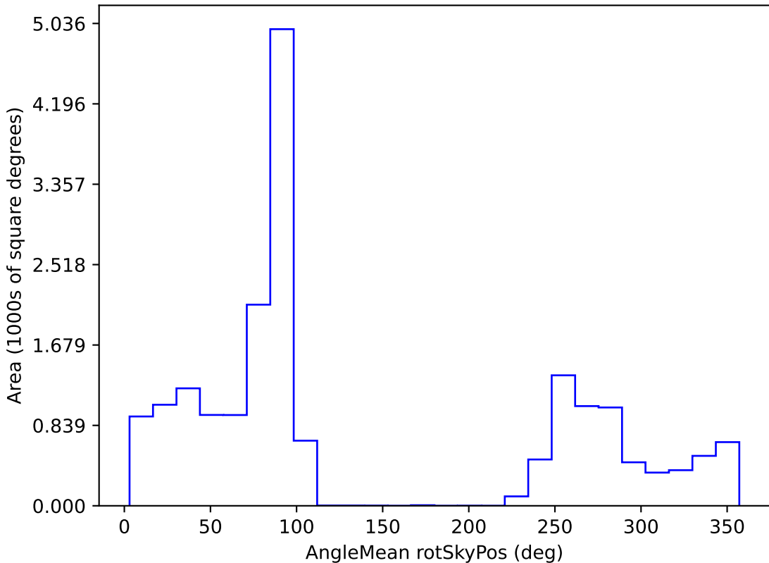
telescope_jerk_v3.5_10yrs WFD all bands: AngleMean rotSkyPos
