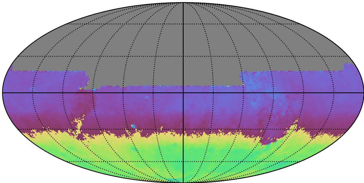
telescope_jerk_v3.5_10yrs All sky y band: AngleMean rotSkyPos
