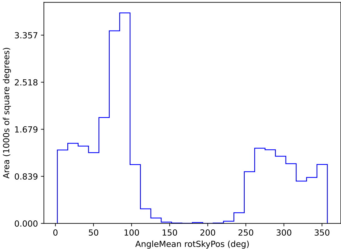
telescope_jerk_v3.5_10yrs All sky y band: AngleMean rotSkyPos
