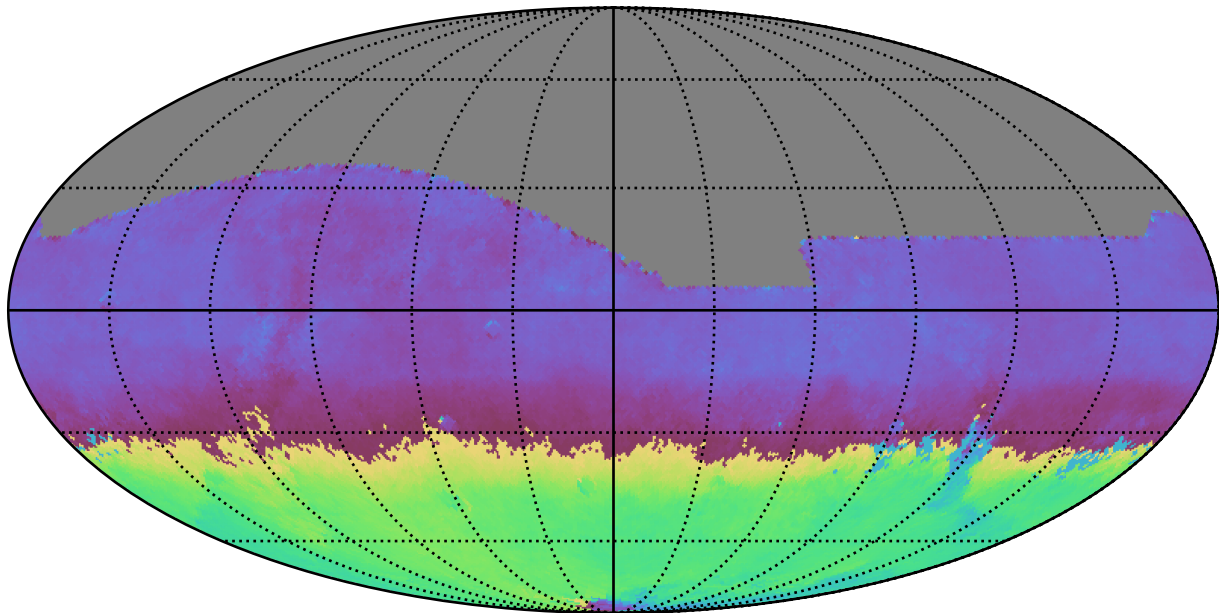
telescope_jerk_v3.5_10yrs All sky r band: AngleMean rotSkyPos
