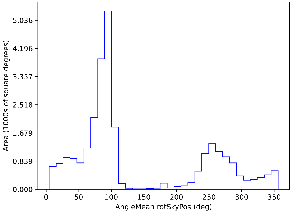
telescope_jerk_v3.5_10yrs All sky r band: AngleMean rotSkyPos
