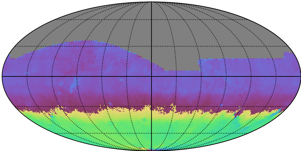
telescope_jerk_v3.5_10yrs All sky i band: AngleMean rotSkyPos
