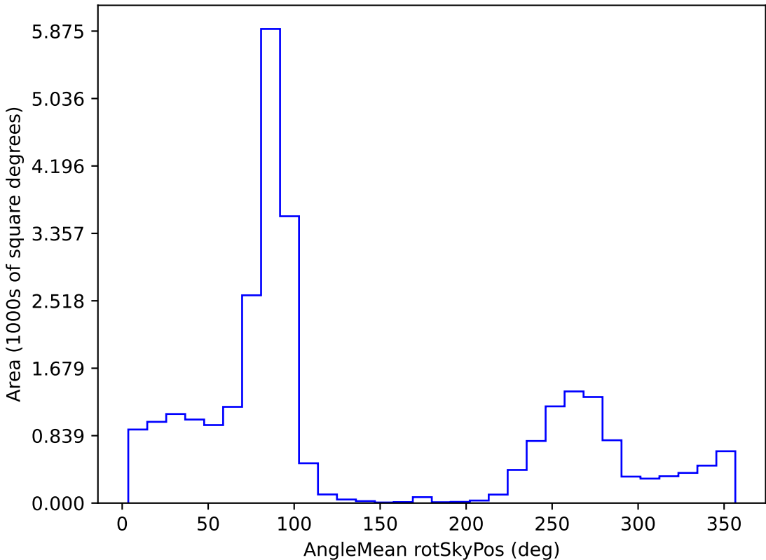
telescope_jerk_v3.5_10yrs All sky i band: AngleMean rotSkyPos
