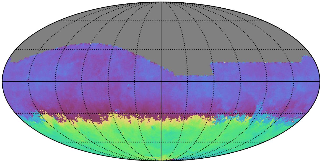
telescope_jerk_v3.5_10yrs All sky g band: AngleMean rotSkyPos
