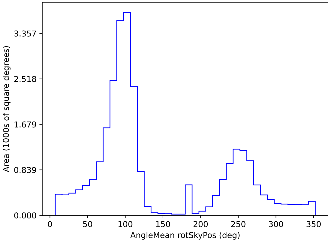
telescope_jerk_v3.5_10yrs All sky g band: AngleMean rotSkyPos
