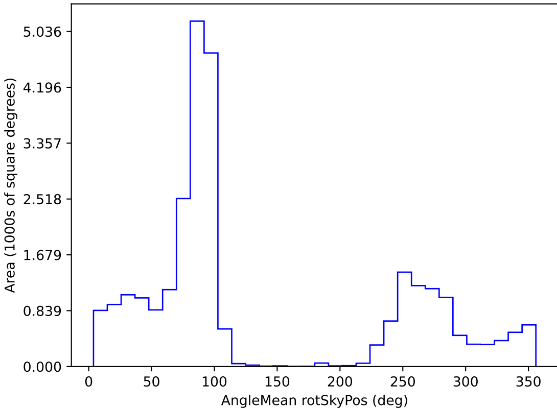
telescope_jerk_v3.5_10yrs All sky all bands: AngleMean rotSkyPos
