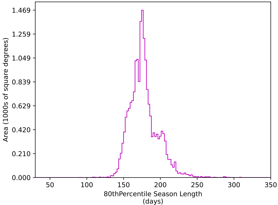
telescope_jerk_v3.5_10yrs WFD z band: 80thPercentile Season Length
