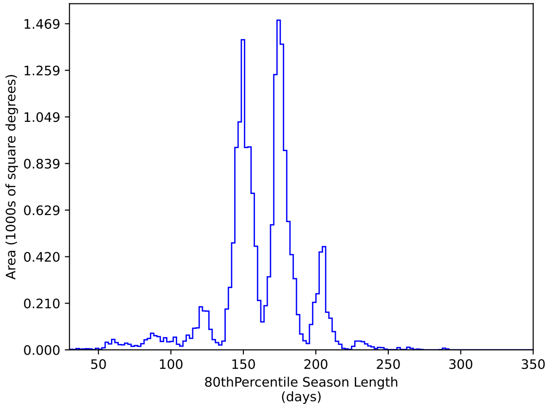
telescope_jerk_v3.5_10yrs WFD y band: 80thPercentile Season Length
