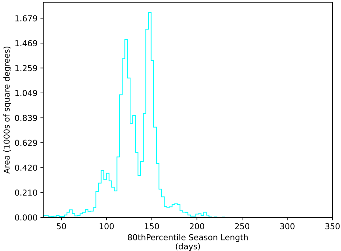
telescope_jerk_v3.5_10yrs WFD u band: 80thPercentile Season Length
