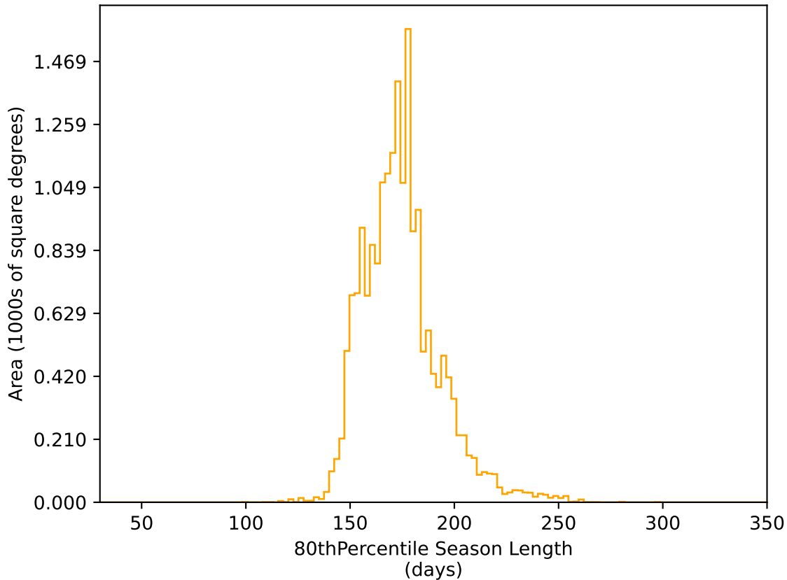
telescope_jerk_v3.5_10yrs WFD r band: 80thPercentile Season Length
