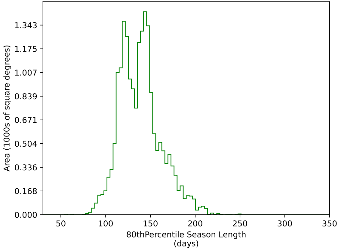
telescope_jerk_v3.5_10yrs WFD g band: 80thPercentile Season Length
