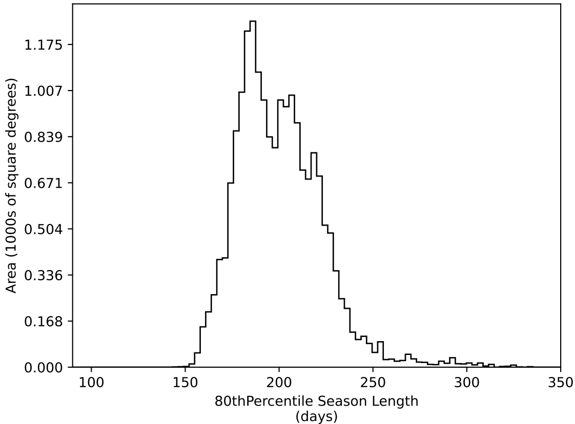
telescope_jerk_v3.5_10yrs WFD all bands: 80thPercentile Season Length
