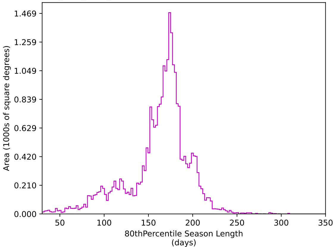
telescope_jerk_v3.5_10yrs All sky z band: 80thPercentile Season Length
