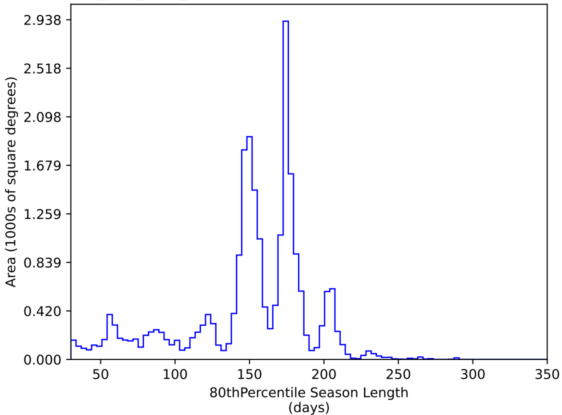
telescope_jerk_v3.5_10yrs All sky y band: 80thPercentile Season Length
