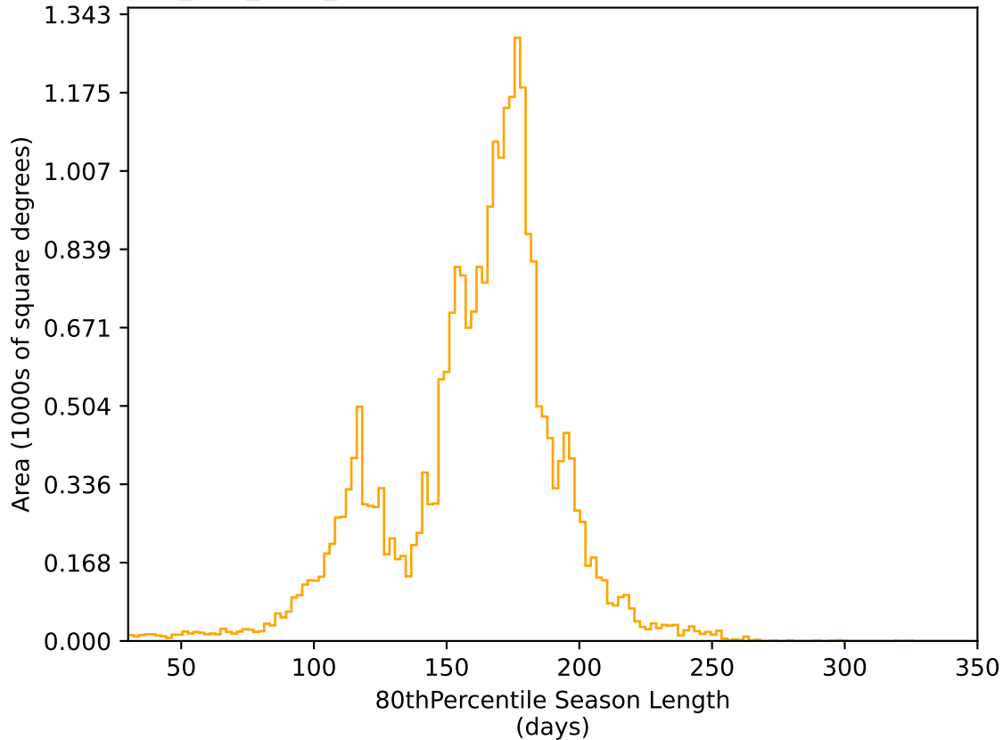
telescope_jerk_v3.5_10yrs All sky r band: 80thPercentile Season Length
