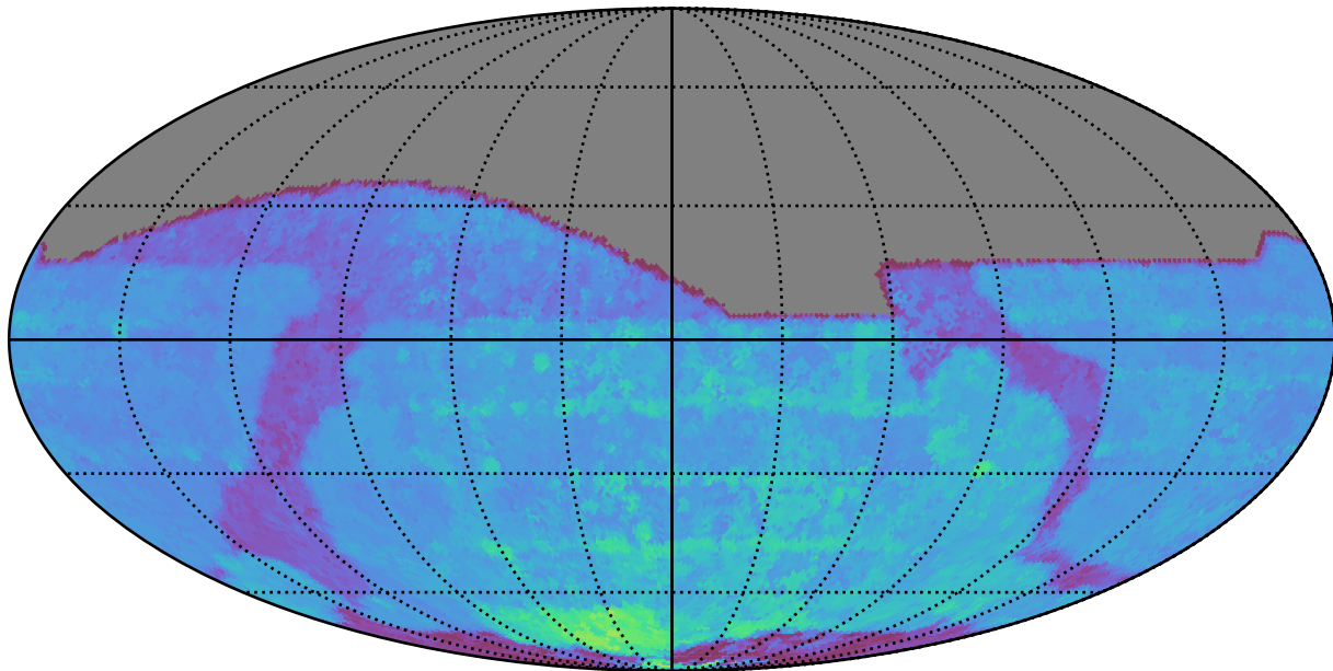
telescope_jerk_v3.5_10yrs All sky i band: 80thPercentile Season Length
