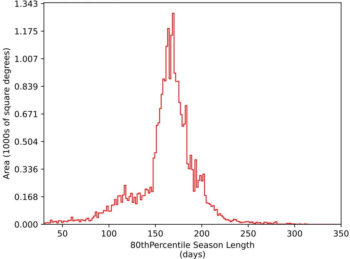
telescope_jerk_v3.5_10yrs All sky i band: 80thPercentile Season Length
