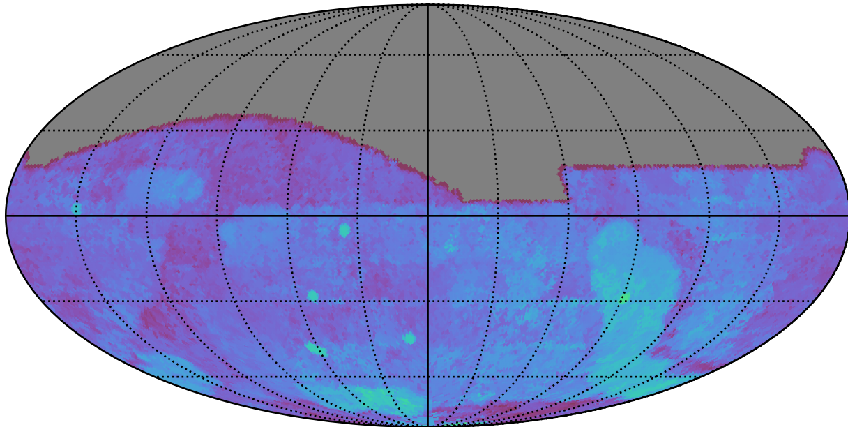
telescope_jerk_v3.5_10yrs All sky g band: 80thPercentile Season Length
