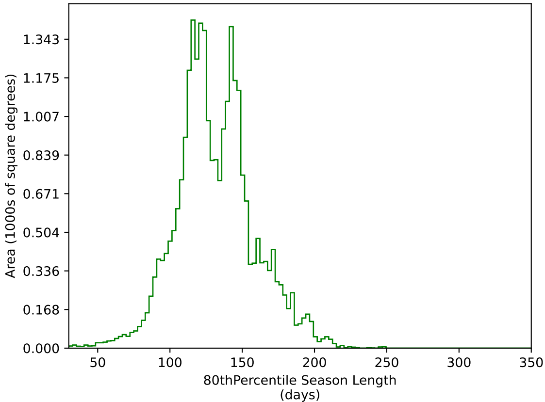
telescope_jerk_v3.5_10yrs All sky g band: 80thPercentile Season Length
