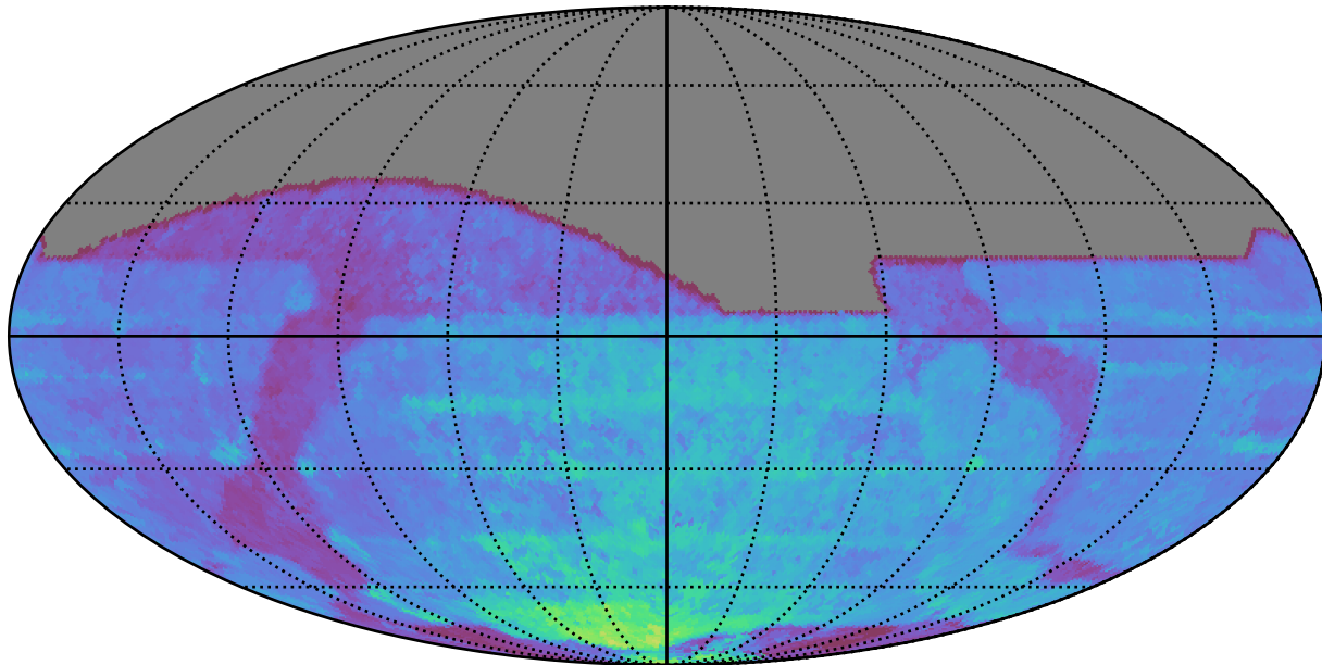
telescope_jerk_v3.5_10yrs All sky all bands: 80thPercentile Season Length
