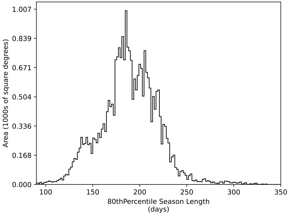
telescope_jerk_v3.5_10yrs All sky all bands: 80thPercentile Season Length
