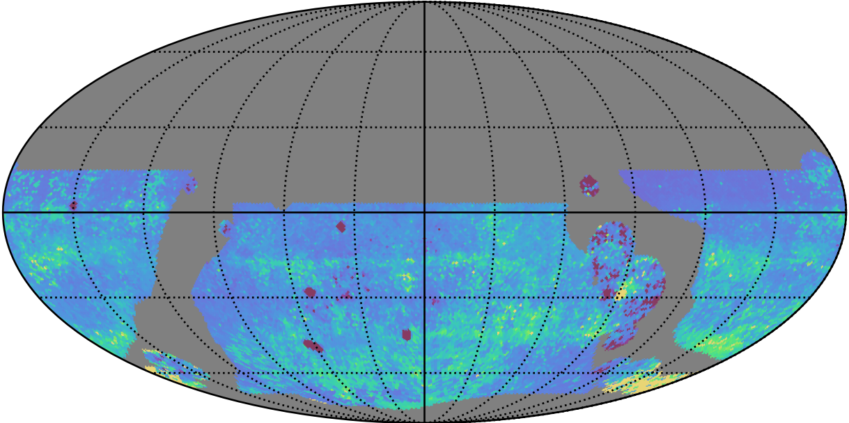
telescope_jerk_v3.5_10yrs WFD zy bands: 75th Percentile Intranight Timespan
