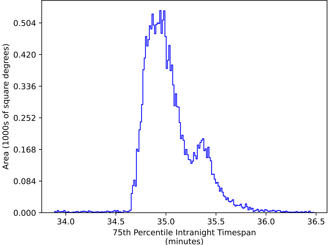
telescope_jerk_v3.5_10yrs WFD zy bands: 75th Percentile Intranight Timespan
