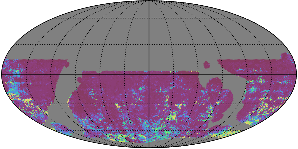
telescope_jerk_v3.5_10yrs WFD z band: 75th Percentile Intranight Timespan
