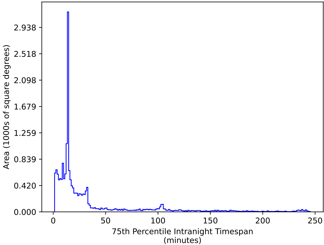
telescope_jerk_v3.5_10yrs WFD z band: 75th Percentile Intranight Timespan
