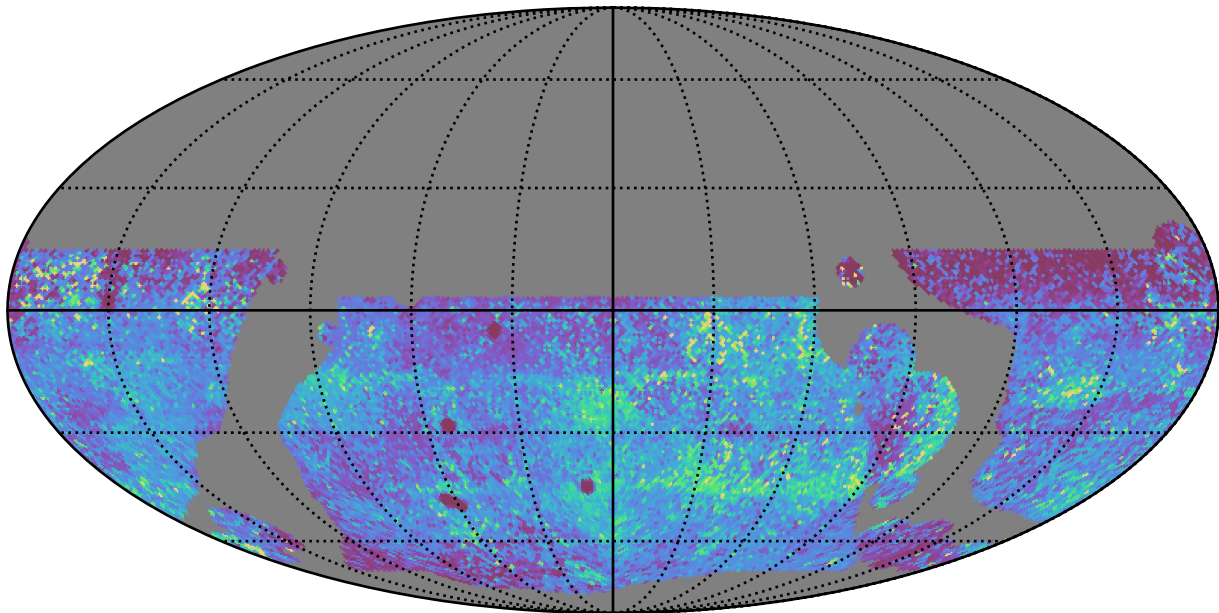
telescope_jerk_v3.5_10yrs WFD y band: 75th Percentile Intranight Timespan
