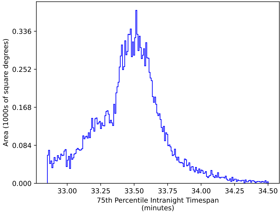
telescope_jerk_v3.5_10yrs WFD y band: 75th Percentile Intranight Timespan
