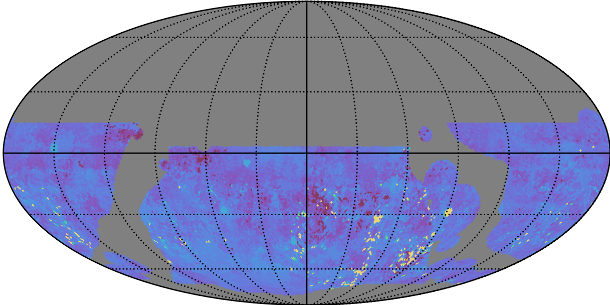
telescope_jerk_v3.5_10yrs WFD ug bands: 75th Percentile Intranight Timespan
