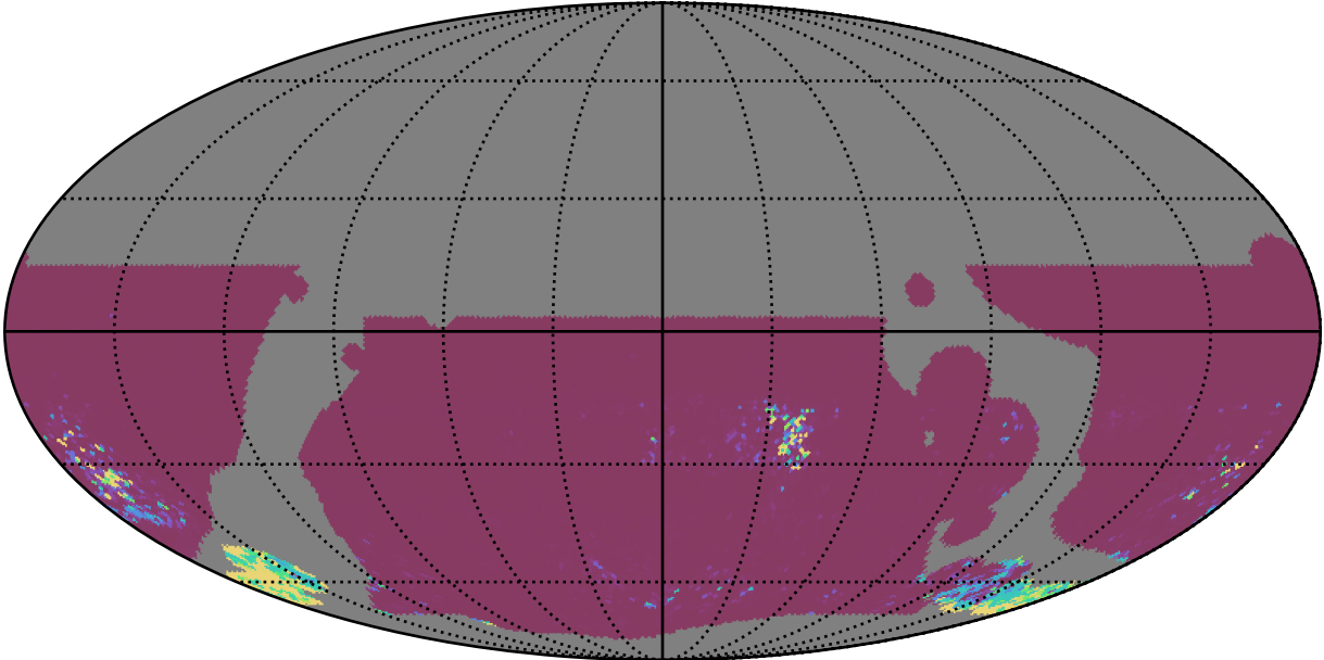
telescope_jerk_v3.5_10yrs WFD ri bands: 75th Percentile Intranight Timespan
