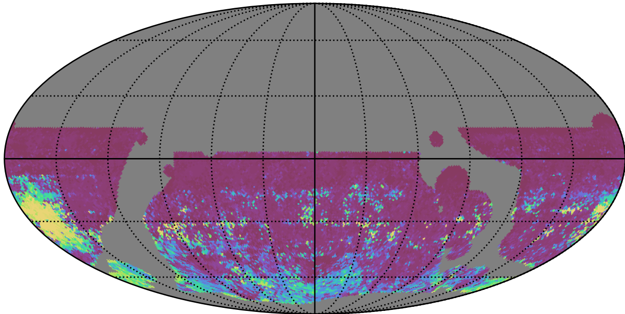
telescope_jerk_v3.5_10yrs WFD r band: 75th Percentile Intranight Timespan
