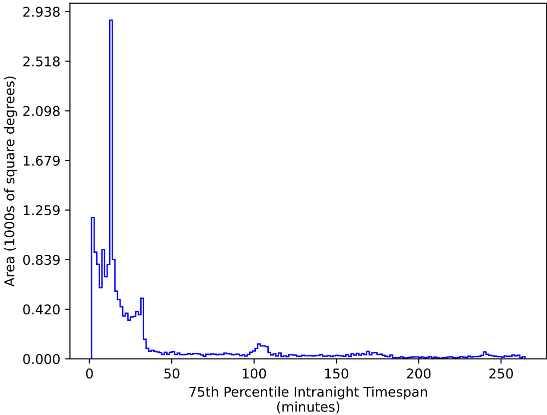
telescope_jerk_v3.5_10yrs WFD r band: 75th Percentile Intranight Timespan
