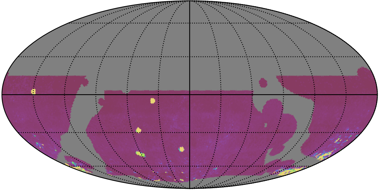
telescope_jerk_v3.5_10yrs WFD iz bands: 75th Percentile Intranight Timespan
