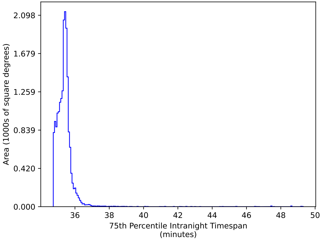
telescope_jerk_v3.5_10yrs WFD iz bands: 75th Percentile Intranight Timespan
