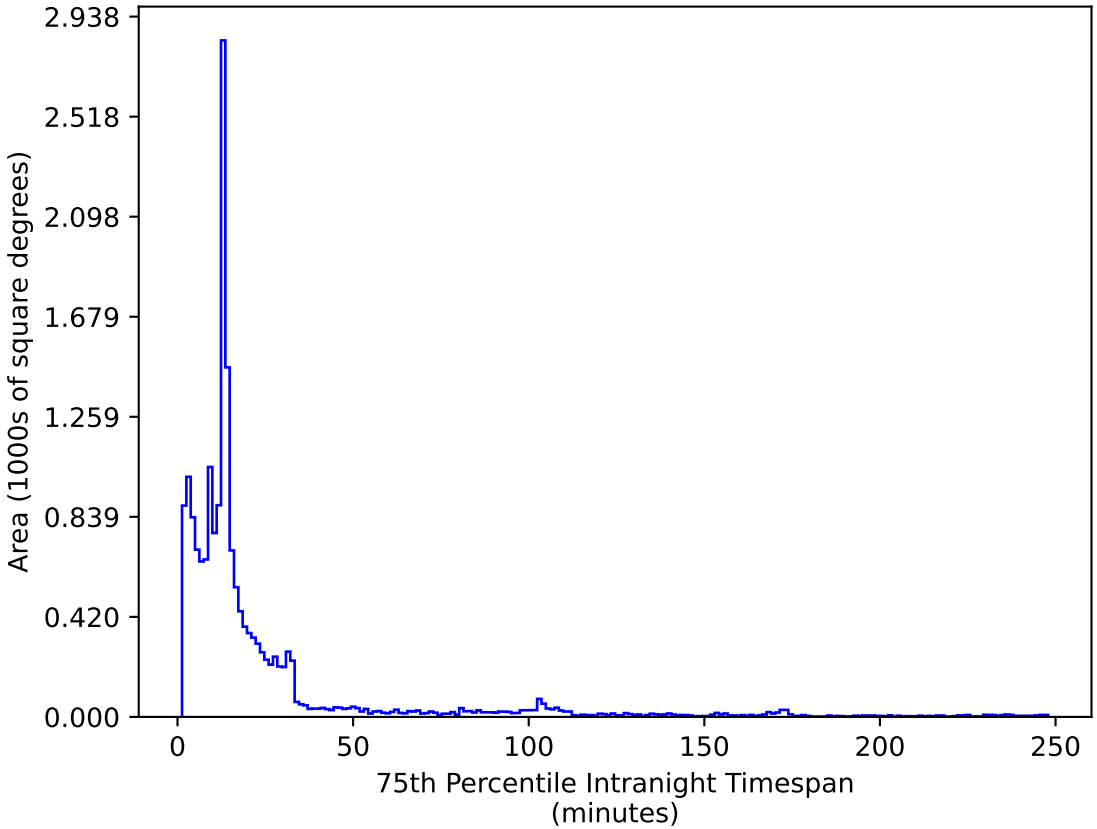
telescope_jerk_v3.5_10yrs WFD i band: 75th Percentile Intranight Timespan
