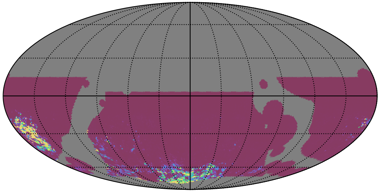
telescope_jerk_v3.5_10yrs WFD gr bands: 75th Percentile Intranight Timespan
