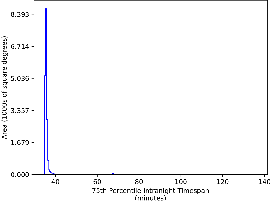
telescope_jerk_v3.5_10yrs WFD gr bands: 75th Percentile Intranight Timespan
