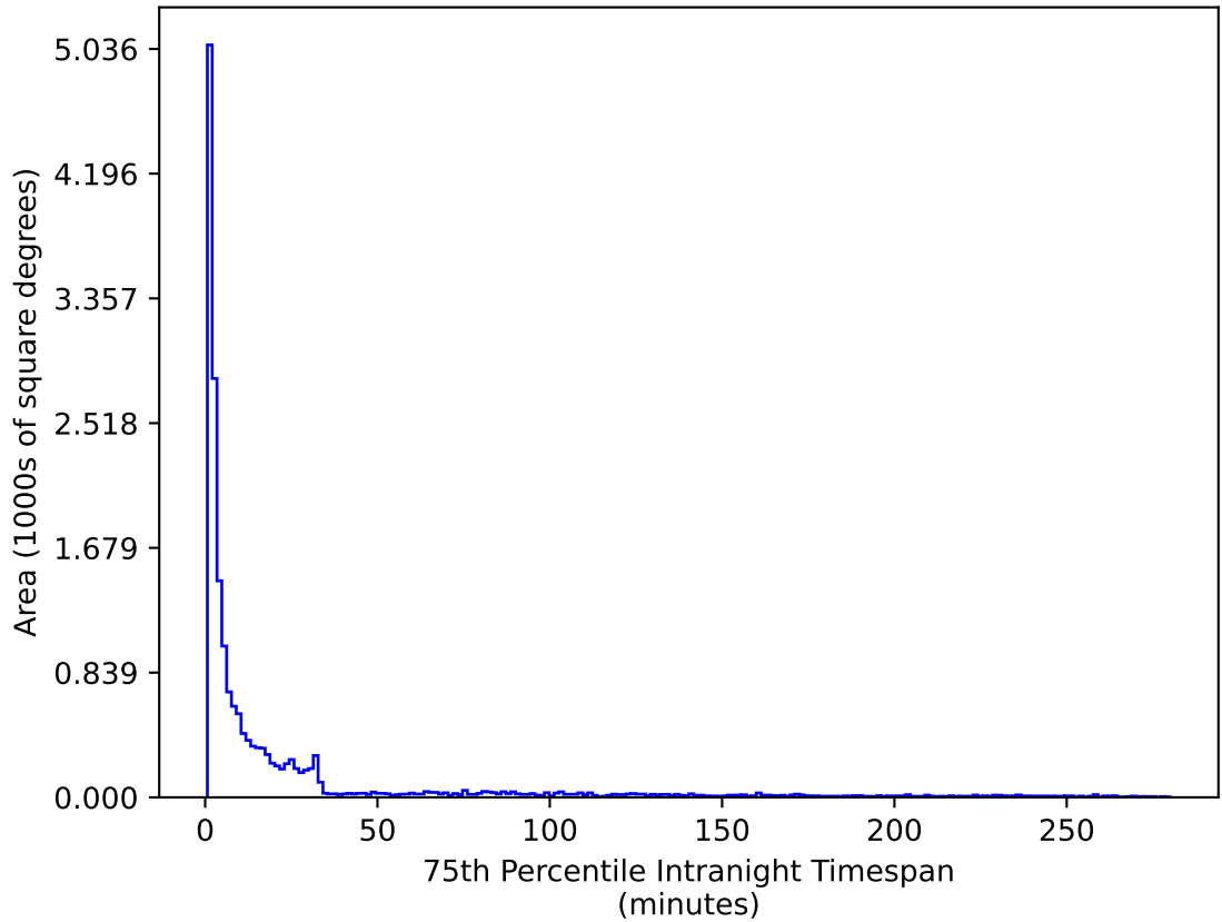
telescope_jerk_v3.5_10yrs WFD g band: 75th Percentile Intranight Timespan
