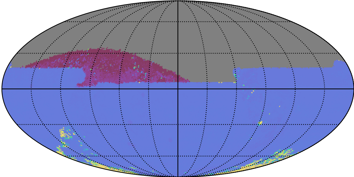
telescope_jerk_v3.5_10yrs All sky zy bands: 75th Percentile Intranight Timespan
