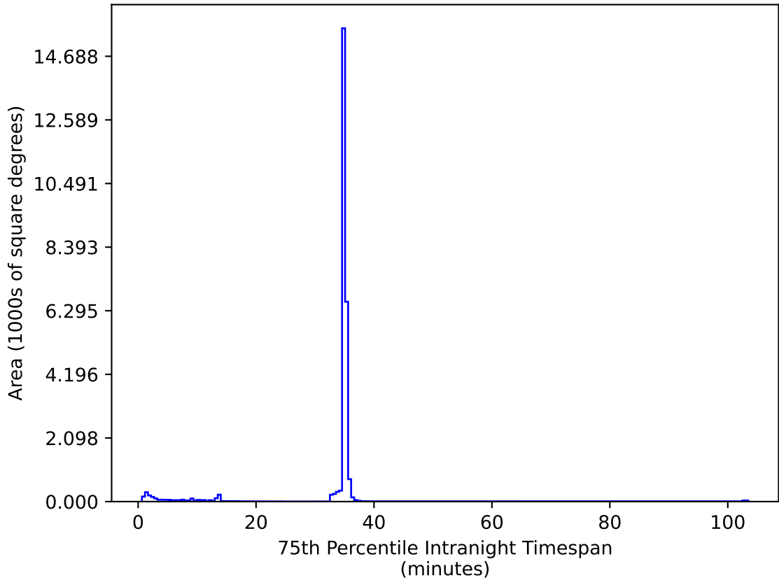
telescope_jerk_v3.5_10yrs All sky zy bands: 75th Percentile Intranight Timespan
