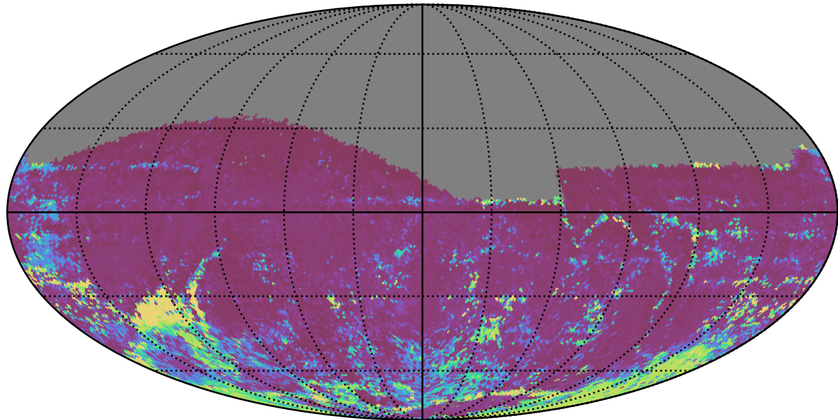
telescope_jerk_v3.5_10yrs All sky z band: 75th Percentile Intranight Timespan
