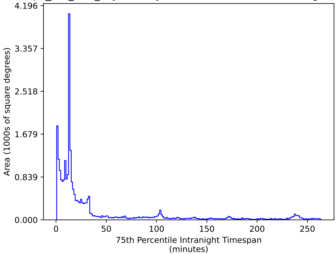
telescope_jerk_v3.5_10yrs All sky z band: 75th Percentile Intranight Timespan
