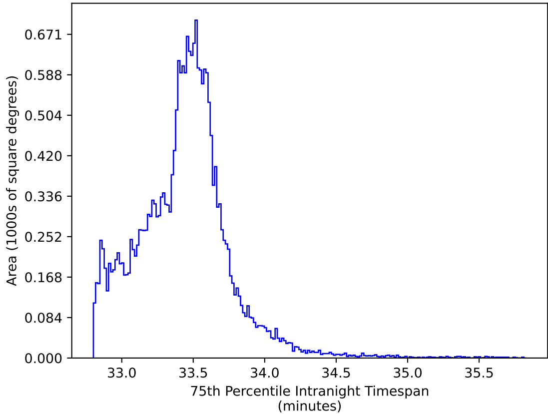
telescope_jerk_v3.5_10yrs All sky y band: 75th Percentile Intranight Timespan
