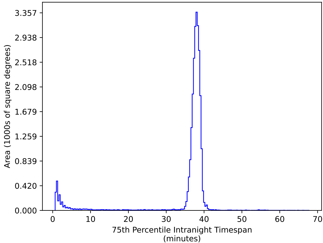
telescope_jerk_v3.5_10yrs All sky ug bands: 75th Percentile Intranight Timespan
