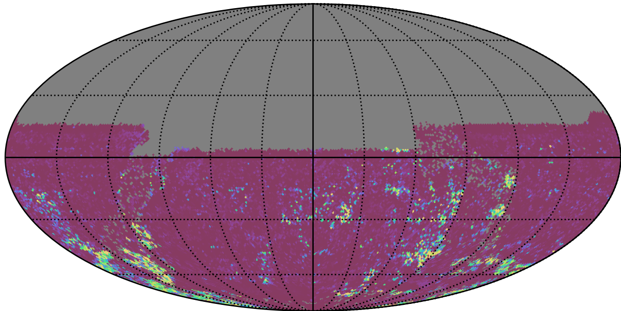
telescope_jerk_v3.5_10yrs All sky u band: 75th Percentile Intranight Timespan
