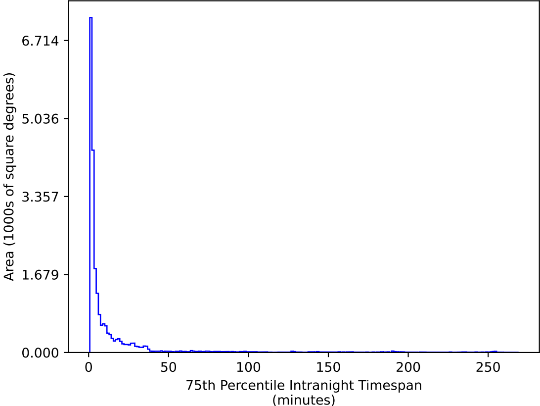
telescope_jerk_v3.5_10yrs All sky u band: 75th Percentile Intranight Timespan
