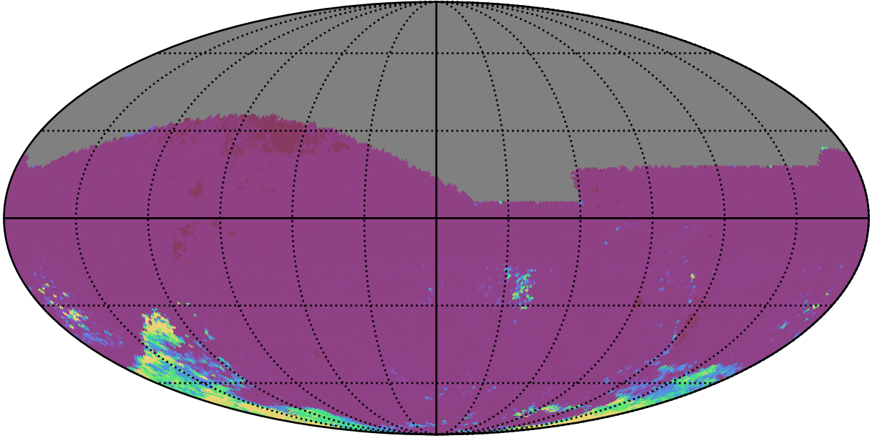
telescope_jerk_v3.5_10yrs All sky ri bands: 75th Percentile Intranight Timespan
